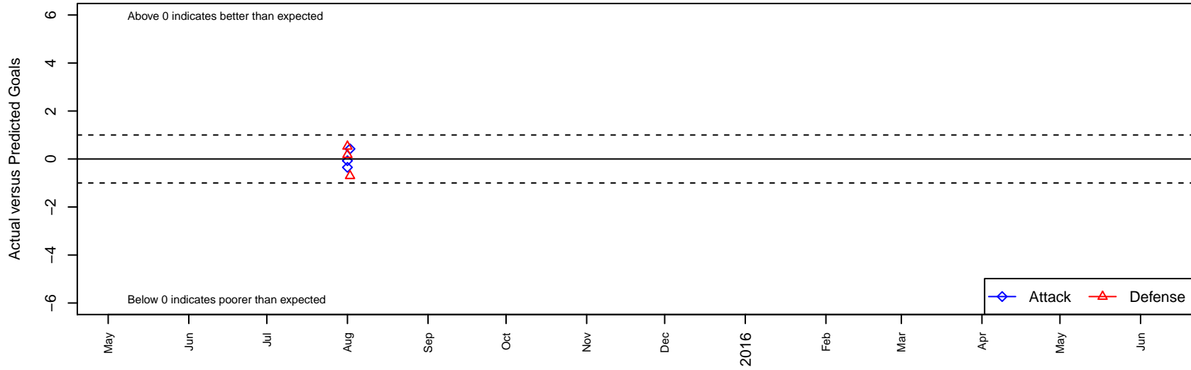
San Jose Earthquakes Pre-Academy B03 Dots are actual minus expected GF (blue circles) and GA (red triangles). Blue line is smoothed change in attack strength. Red is smoothed change in defense strength.
